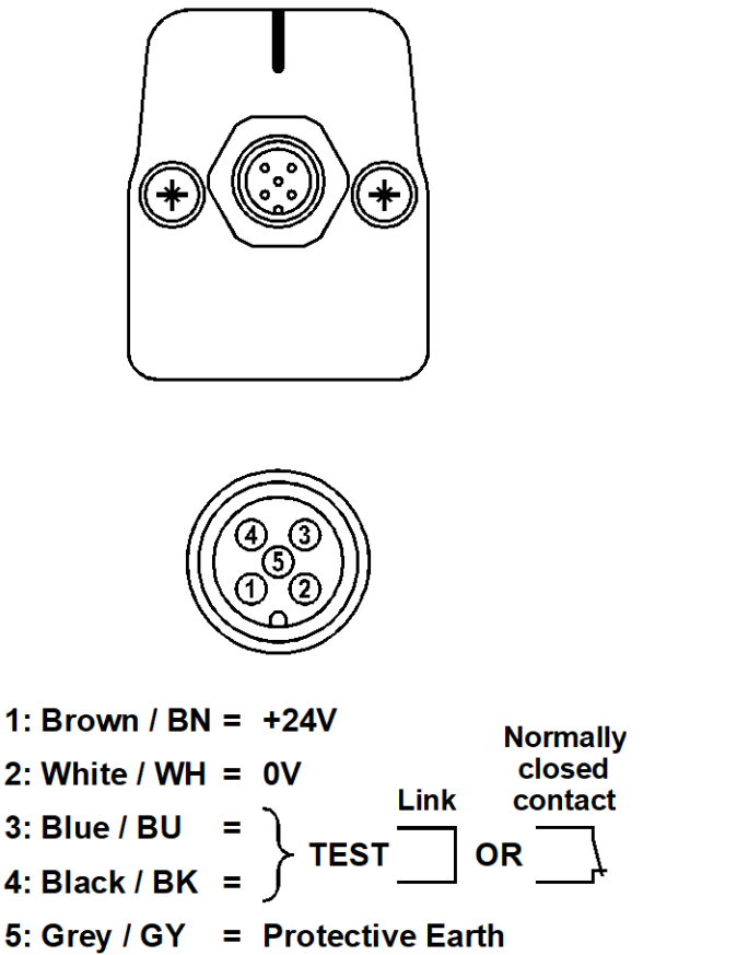
Figure 14 Emitter Unit Connection
