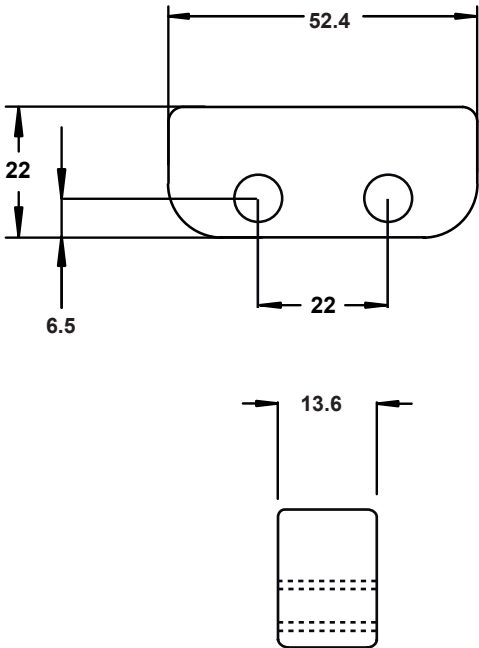
ODNK/OHE1 ACTUATOR
