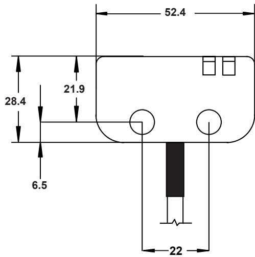
ODNK/OHE1 SWITCH
