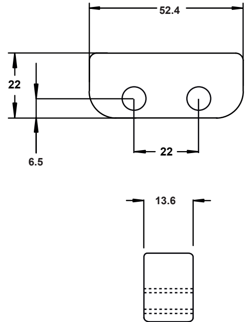
ODNK/OHE1 ACTUATOR
