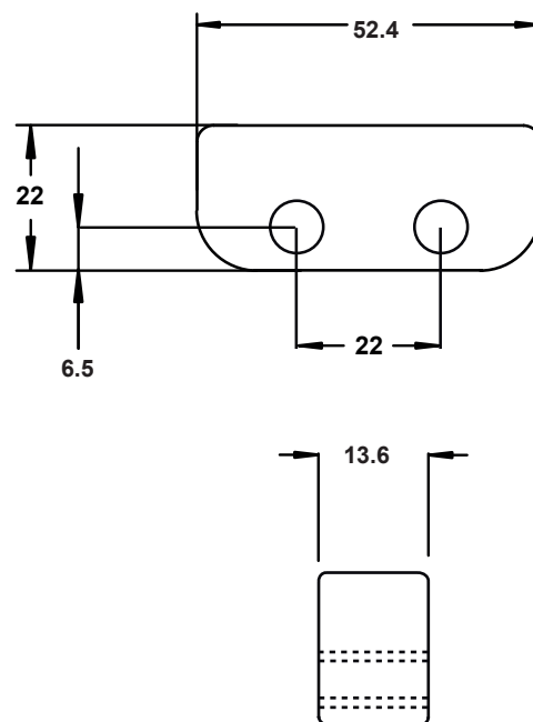
ODNK/OHE1 ACTUATOR
