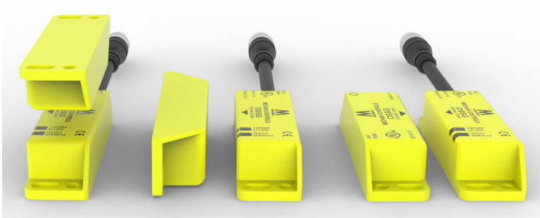
OSSG operates on three faces
