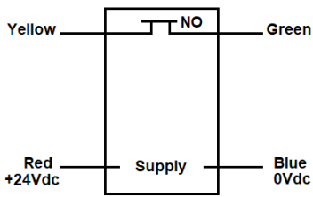
HE1 Contacts 1NO
