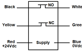
HE1 / HE2 Contacts 1NO + 1NC
