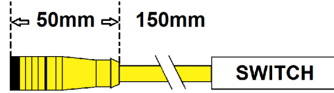
M12 Leaded Quick Disconnect (LQD) HE1 / HE2 / HE6 & HED
