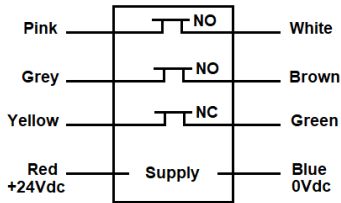
HE1 / HE1-M / HE2 / HE3 / HE4 / HE6 / HEM40 Contacts 2NO + 1NC
