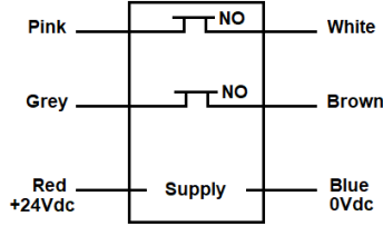
HE1 / HE2 Contacts 2NO
